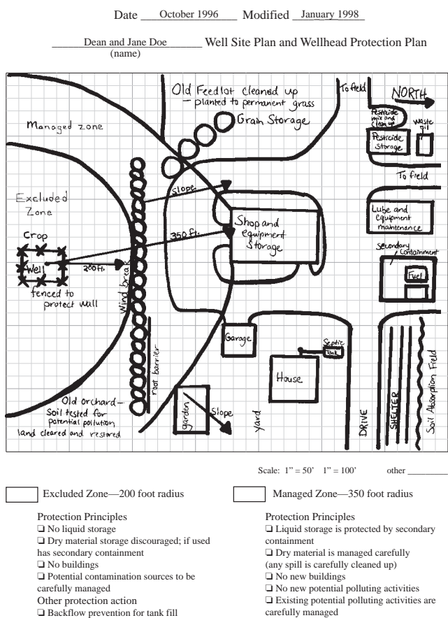
Figure 1. Well Site and Wellhead Protection Plan
